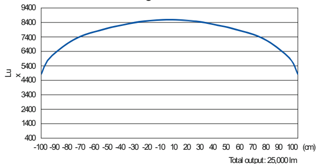
P12 light distribution
