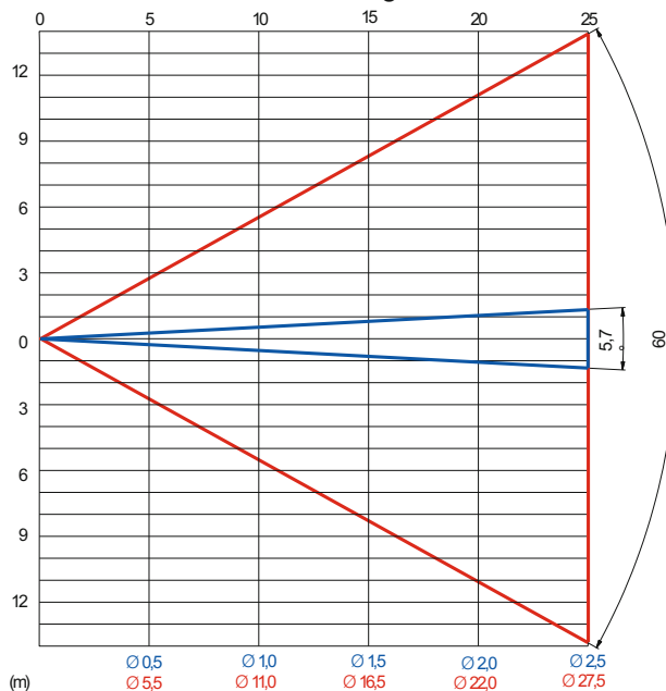
P12 beam angle
